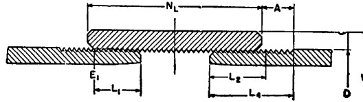
FIG. X1 Dimensions of Hand Tight Assembly for Use with Table X5 FIG. X3.2 Dimensions of Hand Tight Assembly for Use with Table X3.2
