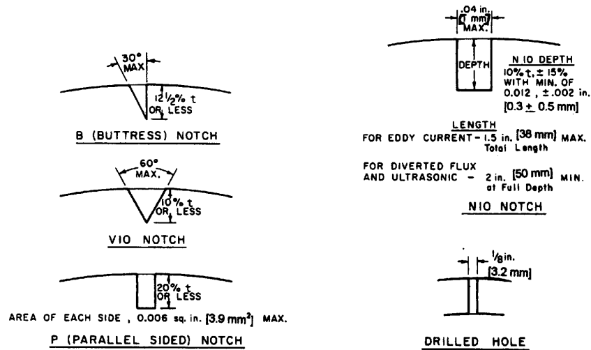
FIG. 1 Calibration Standards
