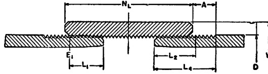
FIG. X1 Dimensions of Hand Tight Assembly for Use with Table X5
